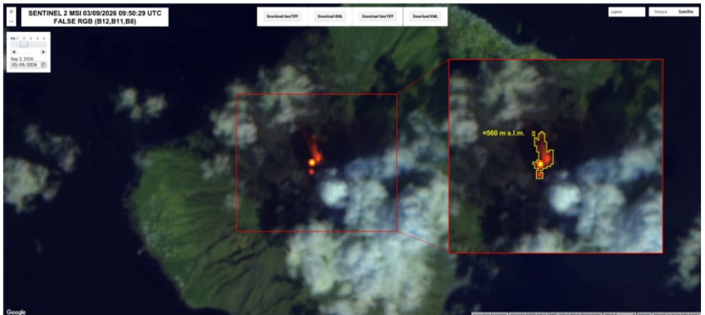
Fig. 7.1 False RGB (Band SWIR2, Band SWIR1 e Band RED) usando Sentinel-2 MSI del 03/09/2026 alle ore 09:50 UTC ( https://www.ct.ingv.it/technolab/v-star ).
